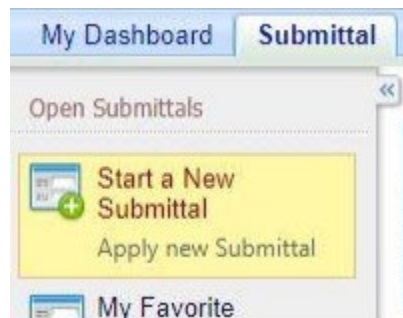
Figure 11 Submittal Menu
